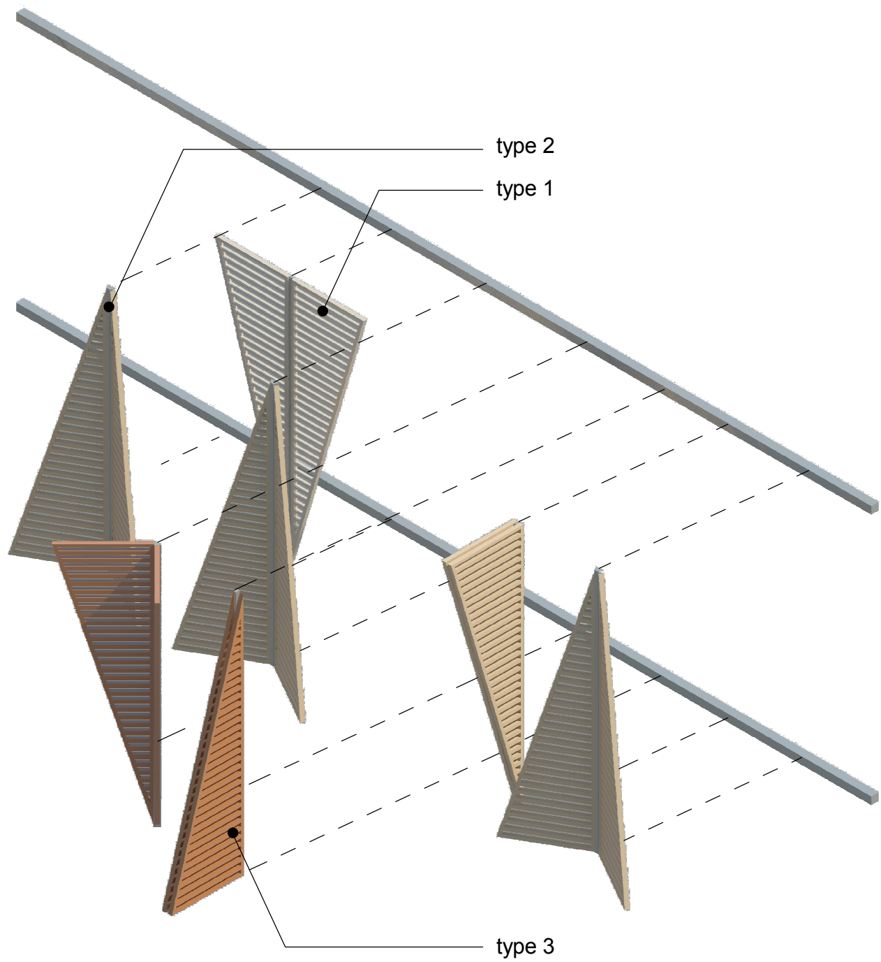
Axonometric exploded view of a facade detail
