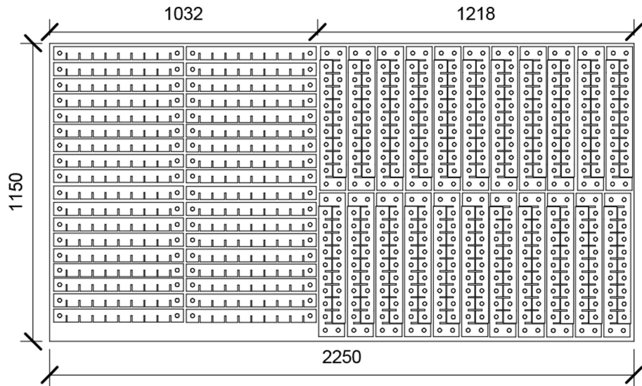
Nesting pannelli 50x50 cm
