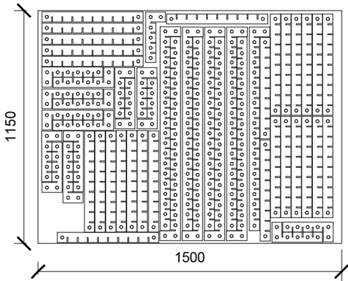
Nesting pannelli 100x50 e 25x50 cm
